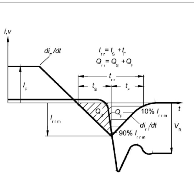
Figure 4. Definition of diode switching characteristics
